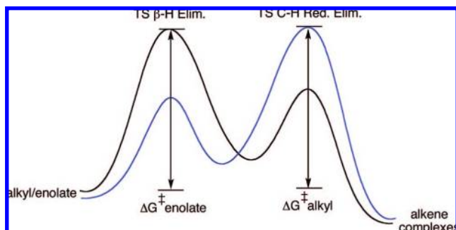
Figure 6. Reaction profiles leading to similar relative rates of elimination from alkylplatinum enolate and alkyl complexes due to a change in the rate-determining step.
