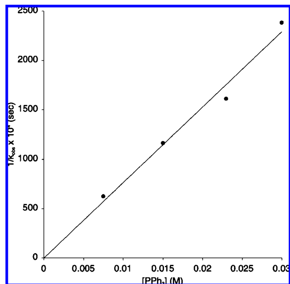
Figure 3. Plot of 1/k_{\text{obs}} vs [\text{PPh}_3] for the thermolysis of p-t -Bu propiophenone-derived enolate 2 in toluene- d_8 at 95^\circ\text{C} .
